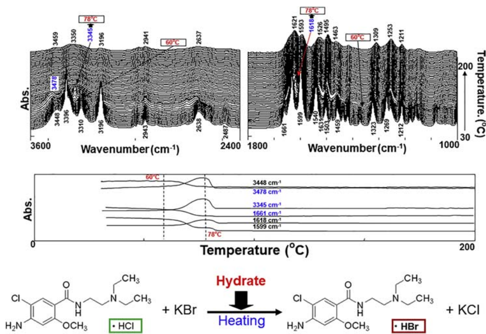
Fig. 9. Three-dimensional FTIR spectral plots and the thermally dependent changes in IR spectra of several specific peaks of metoclopramide hydrochloride monohydrate (MCP HCl \text{H}_2\text{O} ) prepared in the KBr pellet and its pathway of thermally-induced ion-exchange reaction [Modified, with permission from Ref. [166]].
