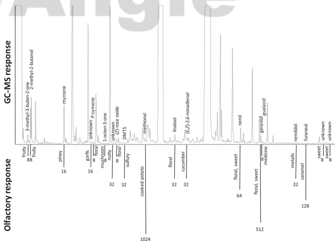
Fig. 2 – GC chromatogram of Sweetheart lychee (SAFE extract) with corresponding identified aroma-active compounds (FD ≥ 8).
