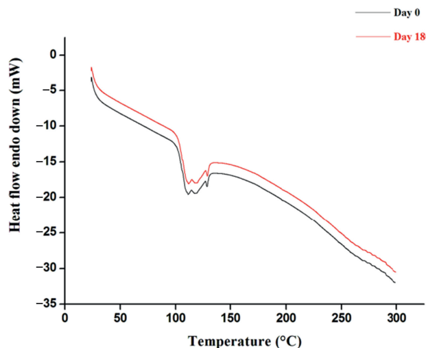
Figure 4 – Differential scanning calorimetry at Day 0 and Day 180.
