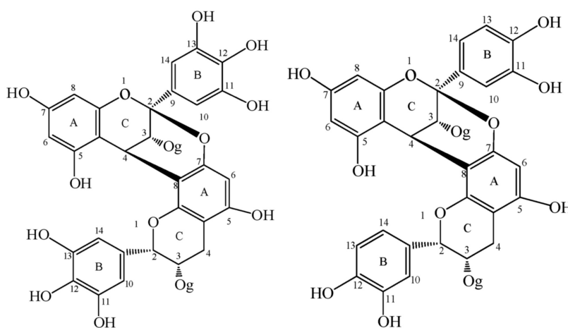
A-type EGCG dimers
