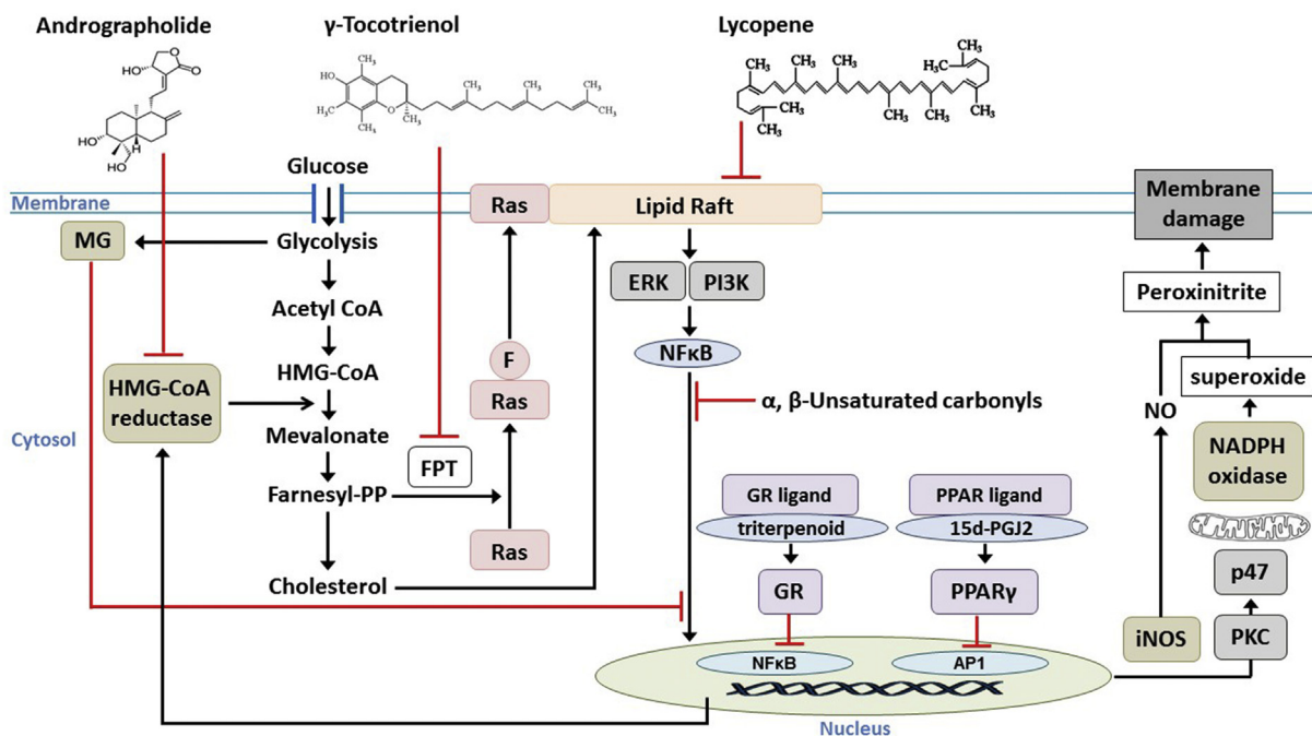
Figure 1 – Multiple targets in macrophage attacked by nutraceuticals. FPT, farnesyl prenyl transferase; MG, methylglyoxal; HMG-CoA, 3-hydroxy-3-methyl-glutaryl-coenzyme A; Farnesyl-PP, farnesyl pyrophosphate; F, farnesyl group; ERK, extracellular signal-regulated kinase; PI3K, phosphoinositide 3-kinase; NF \kappa B, nuclear factor kappa-light-chain-enhancer of activated B cells; GR, glucocorticoid receptor; PPAR \gamma , peroxisome proliferator-activated receptor gamma; AP1, activator protein 1; iNOS, inducible nitric oxide synthase; NO, nitric oxide; PKC, protein kinase C.
