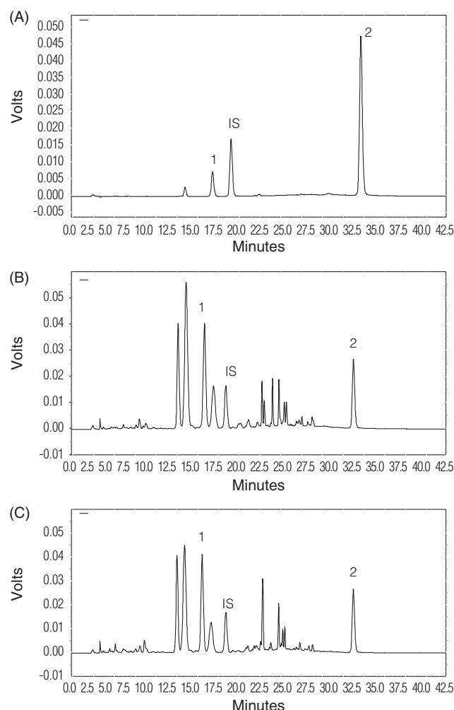
Figure 2. HPLC chromatograms of aloe decoction and its hydrolysate. A: standard; B: aloe decoction; C: aloe hydrolysate. 1: aloin, 2: aloemodin, IS: 6,7-DMC.
