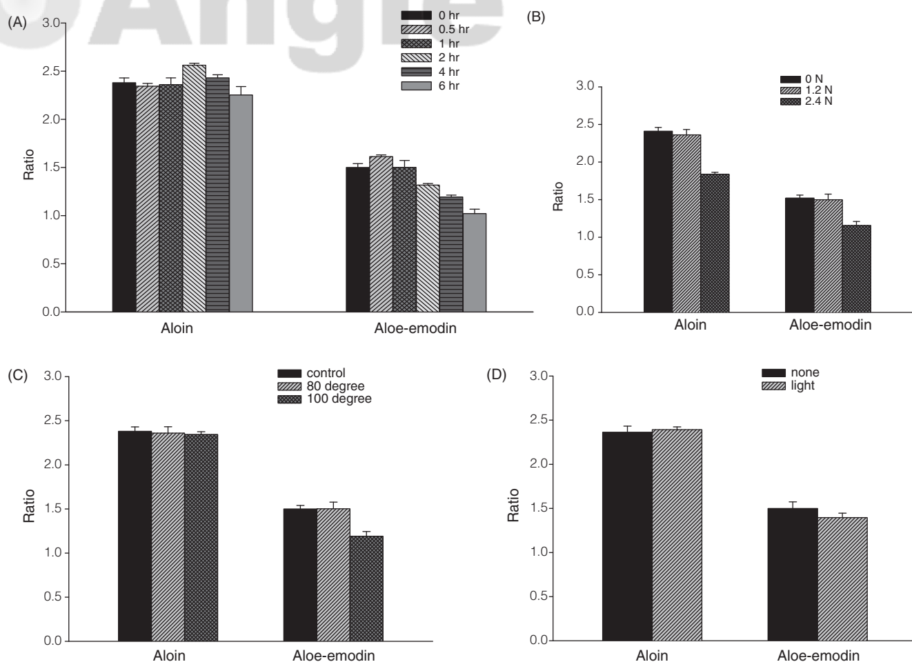
Figure 3. Histograms of aloin-emoedin and aloin contents in aloe decoction after acid hydrolysis. A: the time effect on acid hydrolysis; B: the influence of hydrochloric acid concentration on acid hydrolysis; C: the temperature effect on acid hydrolysis and D: the influence of light on constituents.
