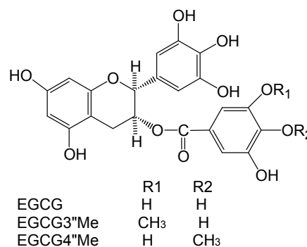
Figure 1. Chemical structure of O -methylated EGCGs and EGCG.
