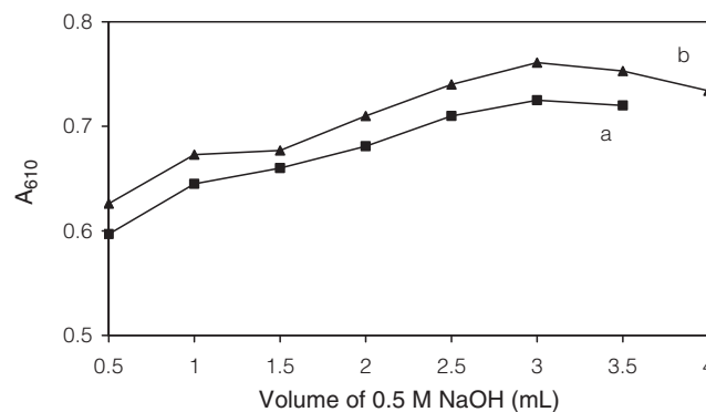
Figure 3. Effect of NaOH concentration on the reaction product of (a) 2.11 × 10 -5 M NF and (b) 3.39 × 10 -5 M VN using optimum conditions for each compound.
