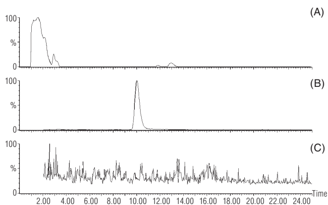
Figure 5. Chromatograms of the selected representative sample. (A) LC-UV chromatogram. (UV = 251 nm), (B) MRM chromatogram of AA-I ( m/z 359>298), (C) MRM chromatogram of AA-II ( m/z 329>268).
