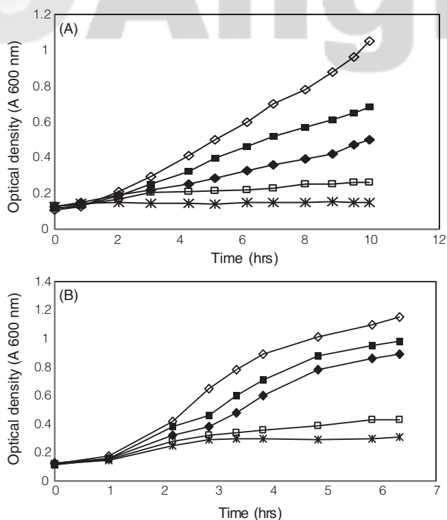
Figure 4. Effect of diallyl sulfide on growth curve of S. mutans 10449 (panel A) and BHT (panel B). Experimental condition as for Figure 3. Symbols: Control ( \diamond ); 0.74 mg/mL ( \blacksquare ); 1.49 mg/mL ( \blacklozenge ); 2.97 mg/mL ( \square ); 5.94 mg/mL (*).
