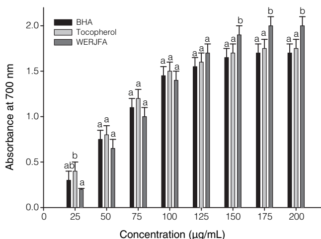
Figure 2. Comparison in reducing capacity of WERJFA, BHA and α-tocopherol at various concentrations. Reducing capacity is shown by absorbance at 700 nm in the ferricyanide reduction test. Data are expressed as means and standard deviations of three independent experiments, each used triplicate samples. Means in the same concentration that don't bear the same superscript were significantly different at 5% level according to Duncan's multiple range test.
