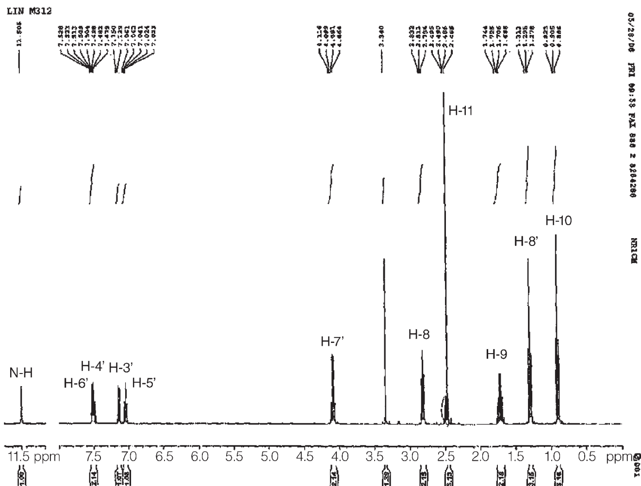
Figure 2. 1 H spectrum of vardenafil analogue A.
