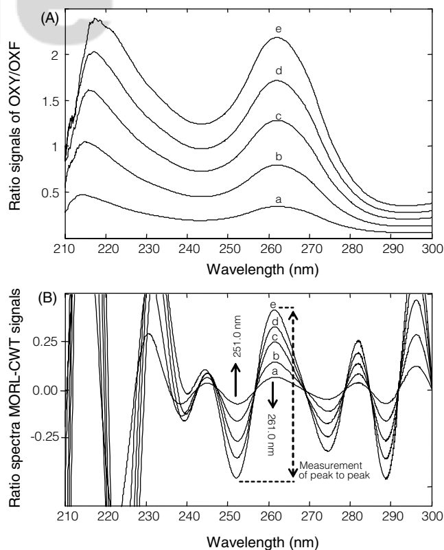
Figure 7. Ratio spectra (A) and their MORL-CWT spectra (B) of (a) 4 µg/mL, (b) 10 µg/mL, (c) 16 µg/mL, (d) 22 µg/mL and 28 µg/mL OXY (when 14 µg/mL OXF was used as a divisor).
