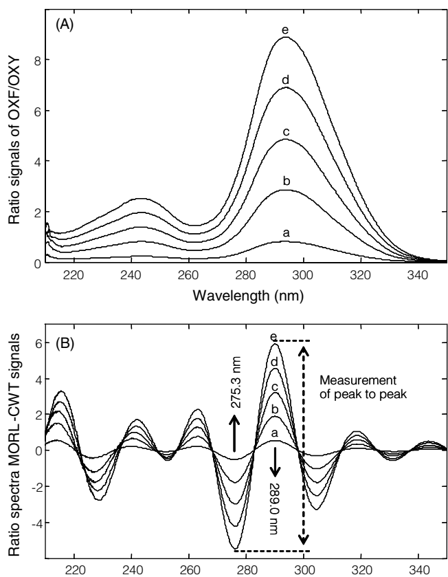
Figure 6. Ratio spectra (A) and their MORL-CWT spectra (B) of (a) 2 µg/mL, (b) 8 µg/mL, (c) 14 µg/mL, (d) 20 µg/mL and 26 µg/mL OXF (when 16 µg/mL OXY was used as a divisor).
