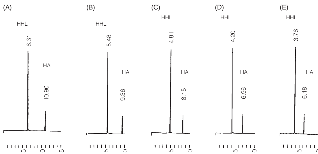
Figure 3. Effect of voltage on the migration times of HHL and HA at varying voltage: (A) 16 kV; (B) 18 kV; (C) 20 kV; (D) 22 kV; (E) 24 kV. Other experimental conditions were as in Figure 2.
