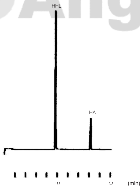
Figure 4. An electropherogram of optimal conditions using the capillary electrophoresis method. (1) standard HHL; (2) standard HA. Experiments were carried out using a fused-silica capillary 65 cm (55 cm to the detector) \times 75 \mu m I.D., 10 mM phosphate buffer at pH 6.0 as the running buffer, an applied voltage of 20 kV, electronic injection time of 2 sec, and a detection wavelength of 228 nm. Sample: a solution of 2.5 mM HA and 2.5 mM HHL in water.
