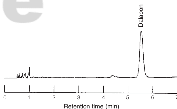
Figure 1. Gas chromatogram of 0.1 μg/mL dalapon methyl ester standard separated with a DB-1 column and detected by an electron capture detector. GC conditions: column temperature, 50°C, 10 min, 30°C/min, 280°C, 3 min; injector temperature, 250°C; detector temperature, 300°C.
