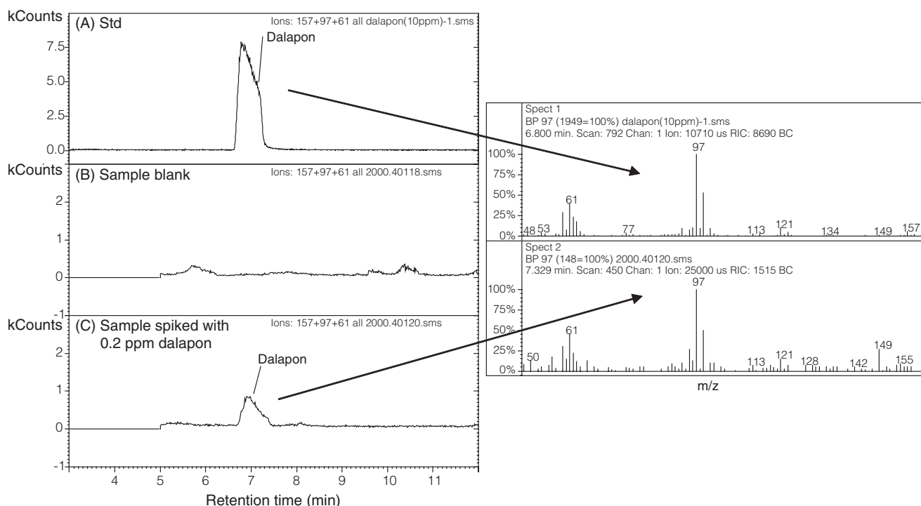
Figure 5. GC-RIC (reconstructed ion current chromatography) of dalapon methyl ester standard (10 \mu\text{g}/\text{mL} ) (A), sugarcane sample blank (B), and sugarcane sample spiked with 0.2 ppm dalapon (C). MS spectra of dalapon methyl ester peak in Figure 5 (A) and Figure 5 (C) are shown on the right.
