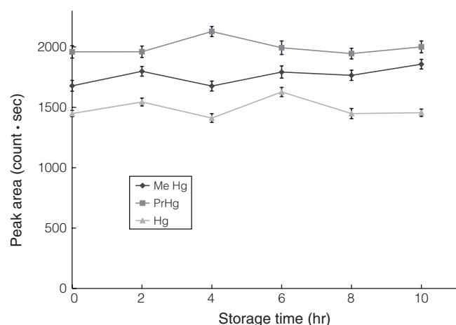
Figure 4. The intra-day stability of 1%NaBPr 4 /KOH of methyl-, propyl-, and inorganic mercury standard solution. Experimental conditions see Table 1.
