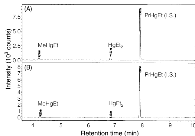
Figure 6. Gas chromatogram of (A) standard solution (1.0 µg/mL as Hg of methyl- and inorganic mercury and 2.0 µg/mL as Hg of propylmercury) and (B) laboratory tuna fish sample (1.98 µg/g methylmercury and 0.20 µg/g inorganic mercury).GC-ITMS conditions see Table 1.
