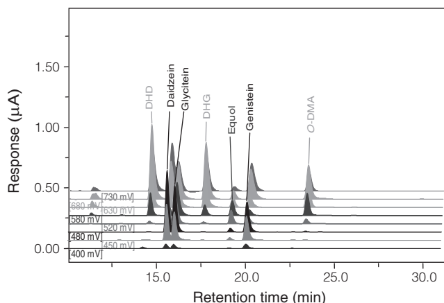
Figure 3. Multi-channel chromatogram of an isoflavone standard mixture (20 ng each) analyzed using HPLC with coulometric array detectors (HPLC-ECD).
