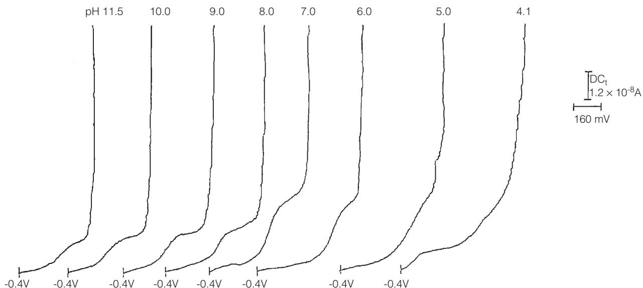
Figure 2. Effect of pH on the development of the polarographic waves of lansoprazole (20 μg mL -1 ) using the anodic DC t mode .
