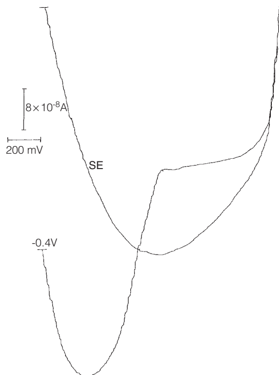
Figure 3. Alternating current behaviour of lansoprazole ( 20 \mu\text{g mL}^{-1} ) in BRb of pH 7. Superimposed alternating voltage: 15 mV; frequency 75 Hz; phase angle 90^\circ . (SE: Supporting Electrolyte).
