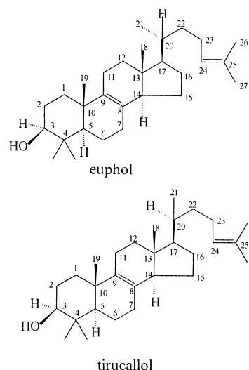
Figure 1. The chemical structures of euphol and tirucallol.
