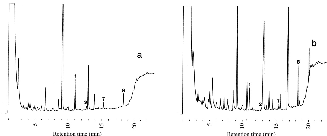
Figure 2. Gas chromatograms of commercial (a) tonic drink and (b) cold formula by direct injection GC method. Peaks : 1 = 1,9-nonanediol (IS), 2 = nicotinamide, 7 = butyl paraben, 8 = caffeine.
