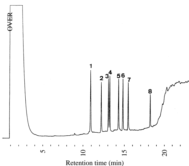
Figure 1. Gas chromatograms of nicotinamide, ethyl-, isopropyl-, propyl-, isobutyl-, butyl-paraben and caffeine authentic standard by direct injection. GC method. Peaks : 1 = 1,9-nonanediol (IS), 2 = nicotinamide, 3 = ethyl paraben, 4 = isopropyl paraben, 5 = propyl paraben, 6 = isobutyl paraben, 7 = butyl paraben, 8 = caffeine.
