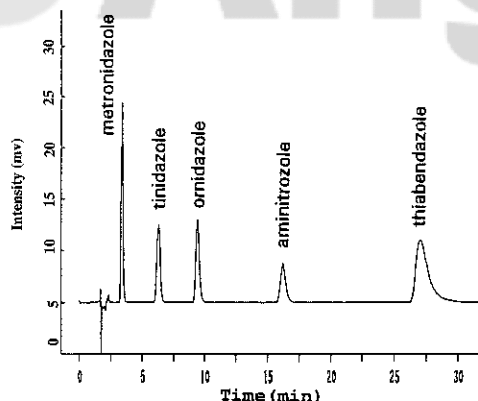
Figure 2. Chromatogram of four antitrichomonal added in Gui-Chi-Hu-Lin-Wan. Thiabendazole was used as internal standard.
