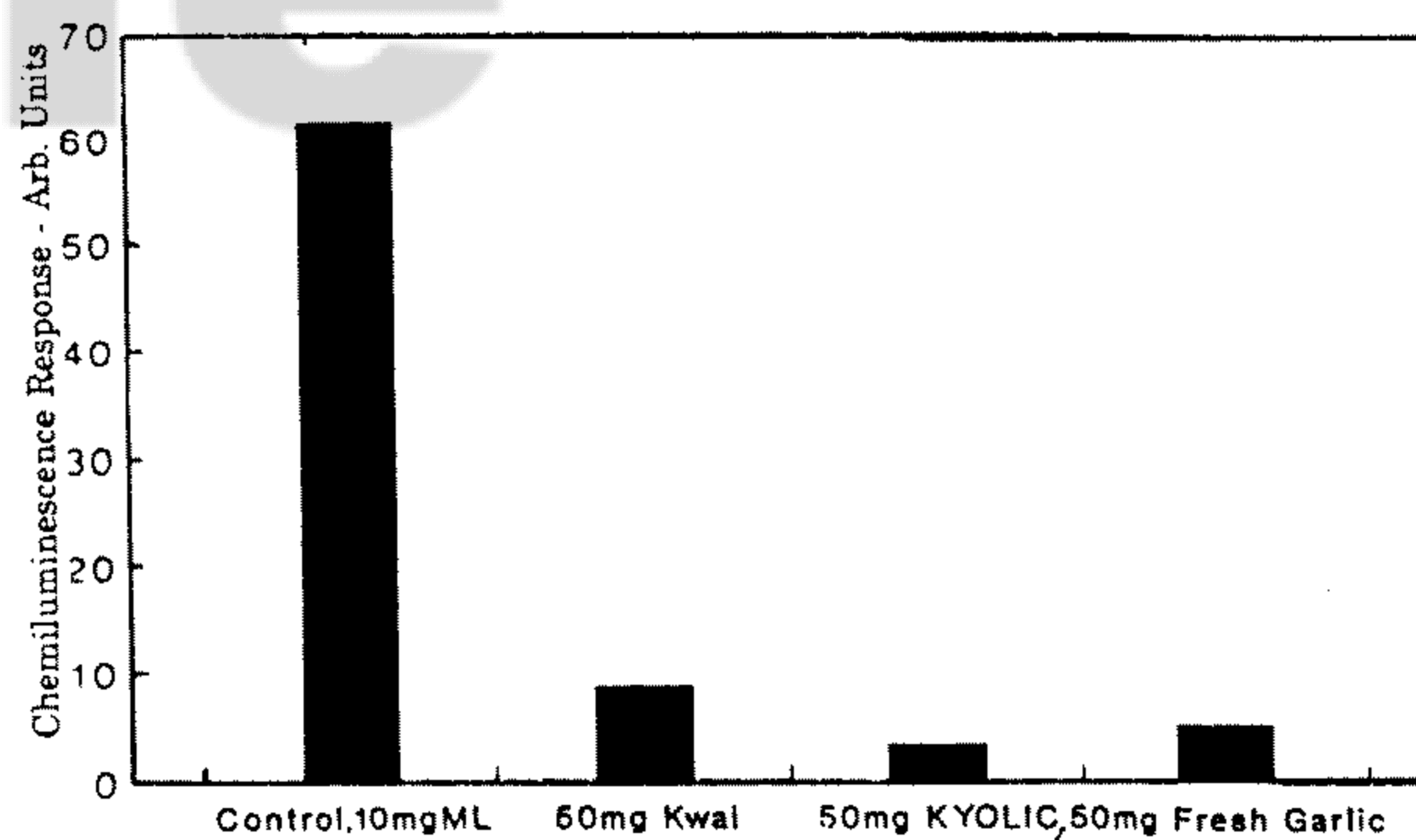
Incubation with methyl linoleate at 60°C for 24.5 hours
