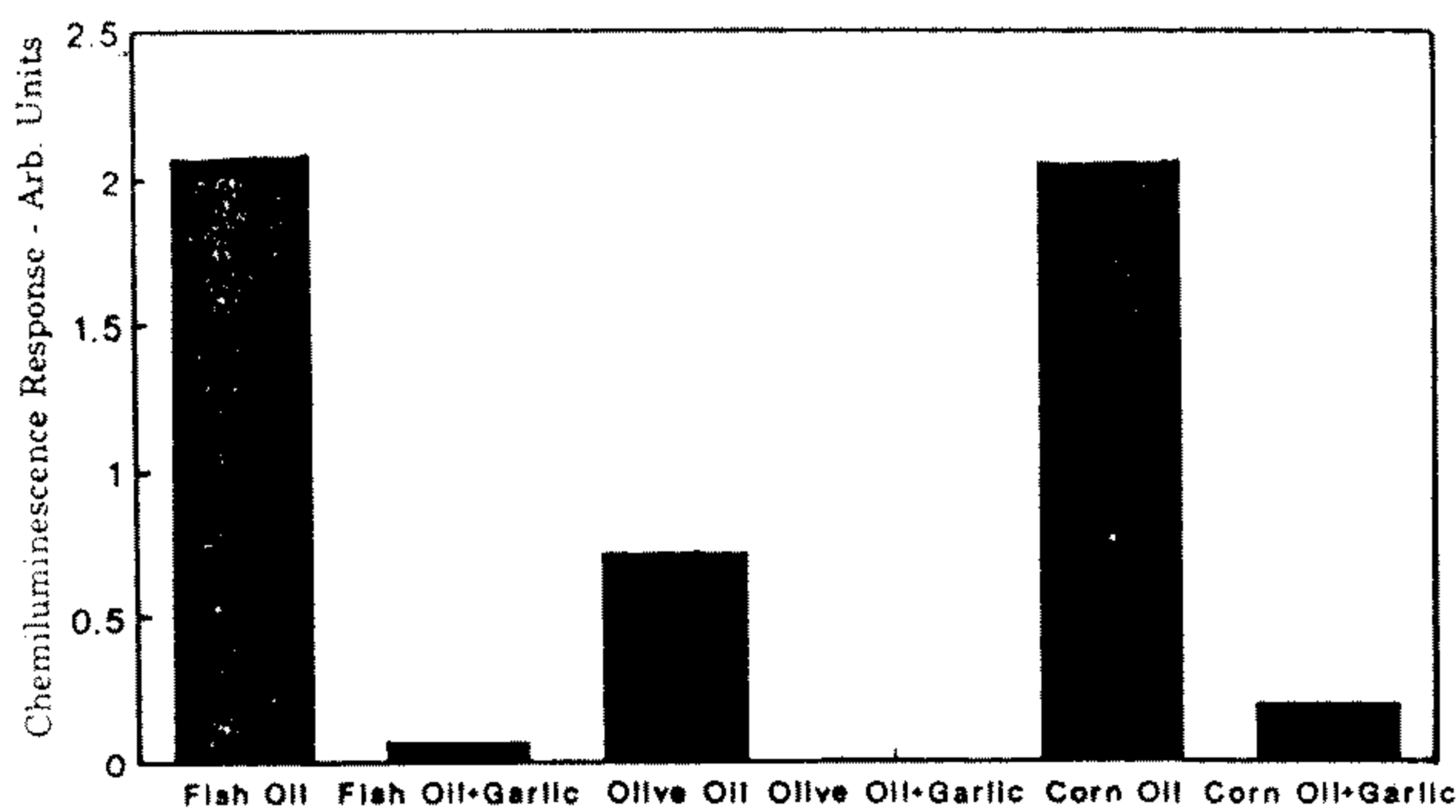
Incubation at 70°C for 20 hours for fish oil and 90 hours for corn and olive oil
