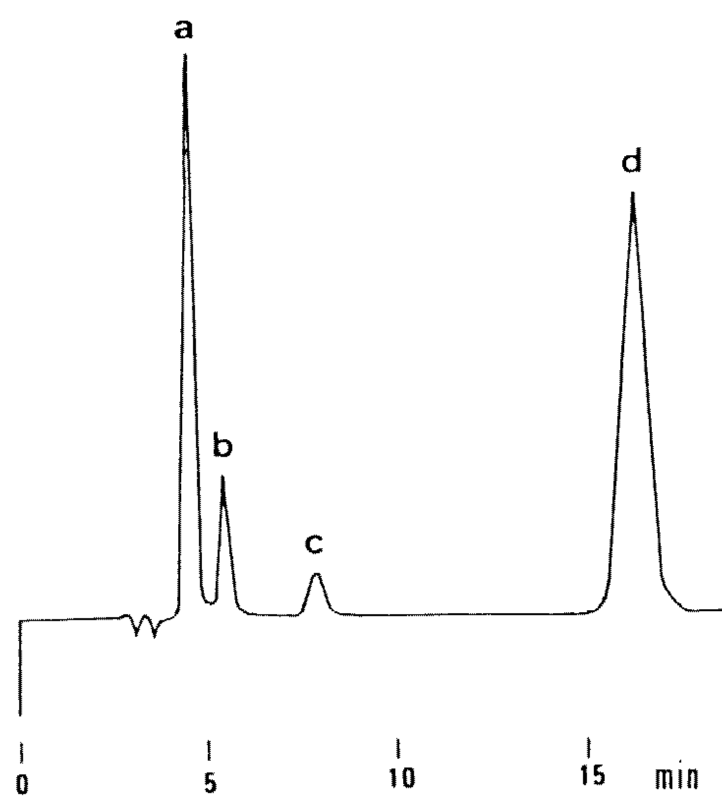
Figure. 1 Liquid chromatogram of a caffeine-ethoxybenzamide-propyphenazone mixture in methanol-acetonitrile 3% aqueous acetic acid (24 : 16 : 60) on a \mu bondapak C18 column at a flow rate of 1 ml min -1 . Key : a, caffeine; b, salicylamide (internal standard); c, ethoxybenzamide; and d, propyphenazone.
